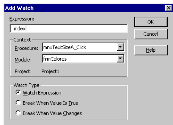
Figura 2.17. Ventana Add Watch .
